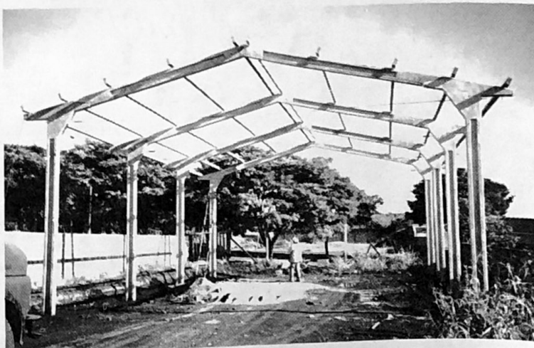
Here you see the strongly built prefab structure of the building in Urai. This is on the front of the lot which measures 45.5 feet by 195 feet. It is the same size as the building in Nova Fatima.
