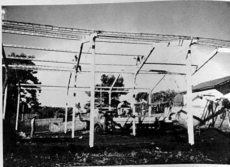
The largest building is in Leopoldina. This lot is 81 feet by 163 feet. The building has a capacity of 300 people. The width of the lot made it possible to put the building sideways and the second part was built for 30% less.
