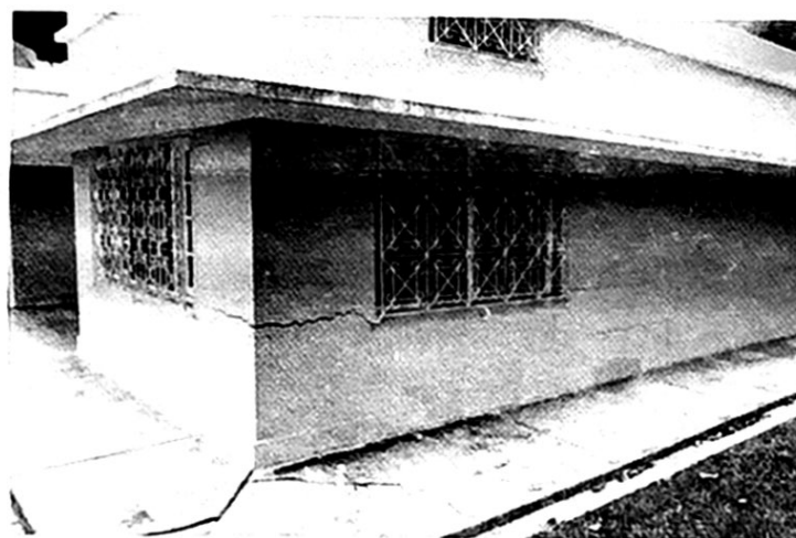
Mayfield house, Pucallpa, Peru. This picture was taken in September (four months ago) and we have just received it with a letter from Brother Gibbs telling about cracks in the building, front, side and rear. Reinforced concrete with steel will have to be put under the walls. We are advised that the damage (caused from settling) is much worse now than when the above picture was taken. Brother Gibbs estimates that this will cost about $2,000.00 to repair. PLEASE HELP NOW.
