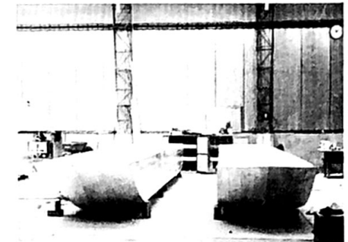
Front view of the two aluminum pontoons that the houseboat will be built on. These pontoons will hold the fuel tanks and also a Diesel engine in the rear of each pontoon.
